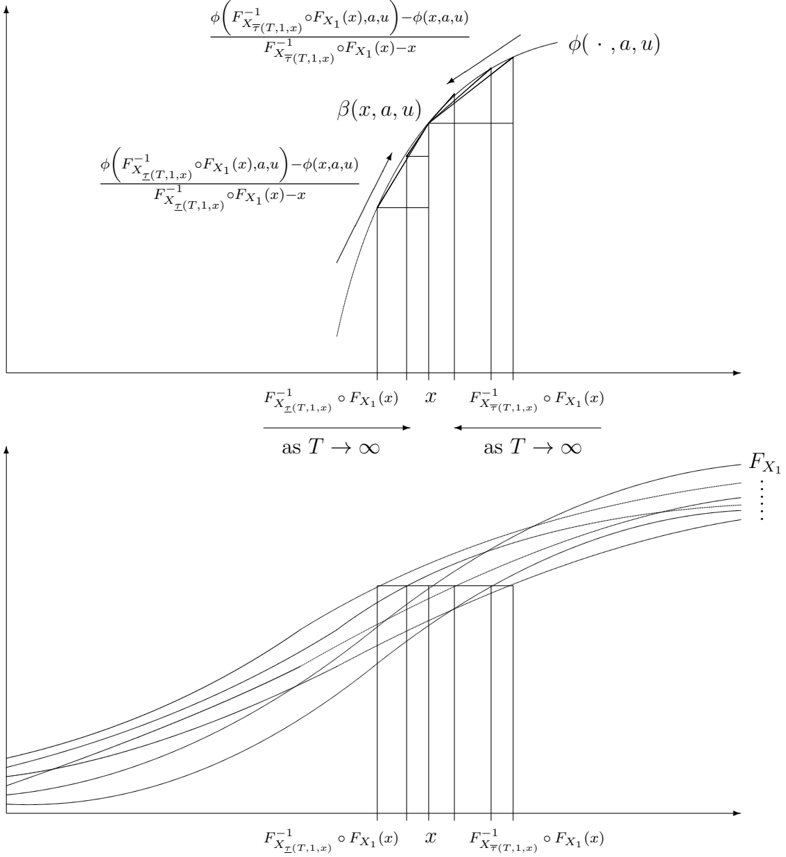
Figure 3: Point identification as T \rightarrow \infty : left/right difference quotients converge to \beta(x, a, u) .
