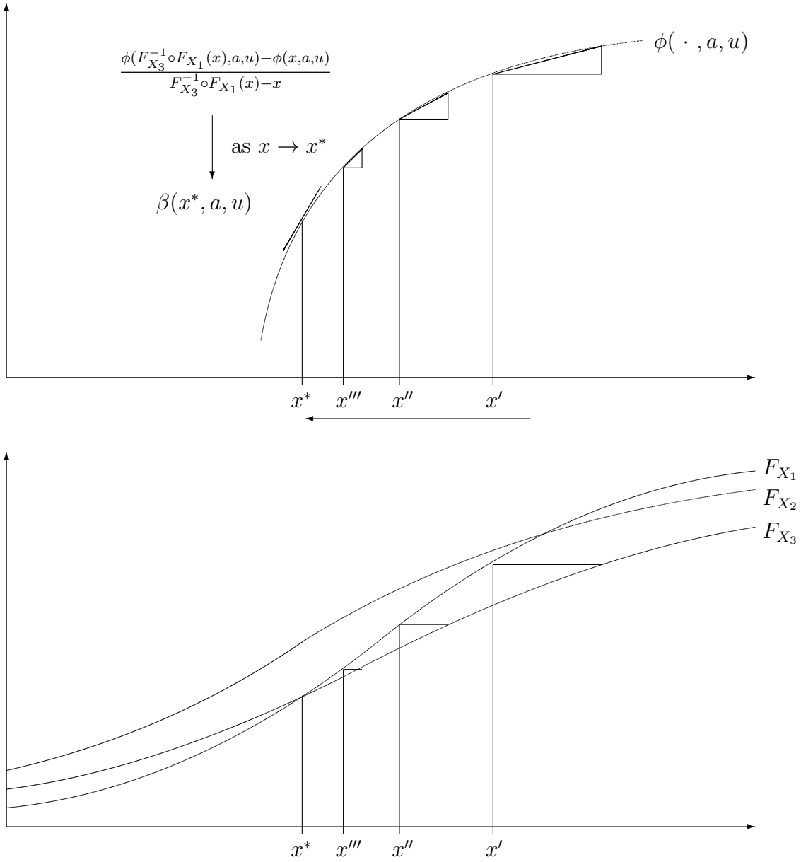
Figure 2: Local point identification under T < \infty : difference quotients converge to \beta(x^*, a, u) .
