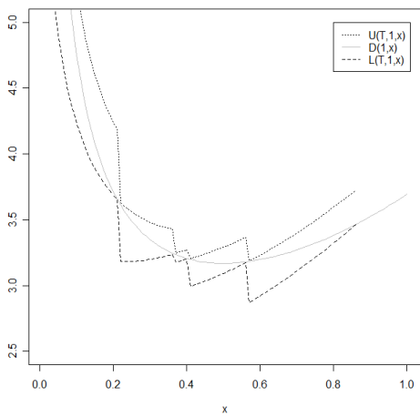
Figure 4: Numerical illustration of transition of identifiability as T rises.
