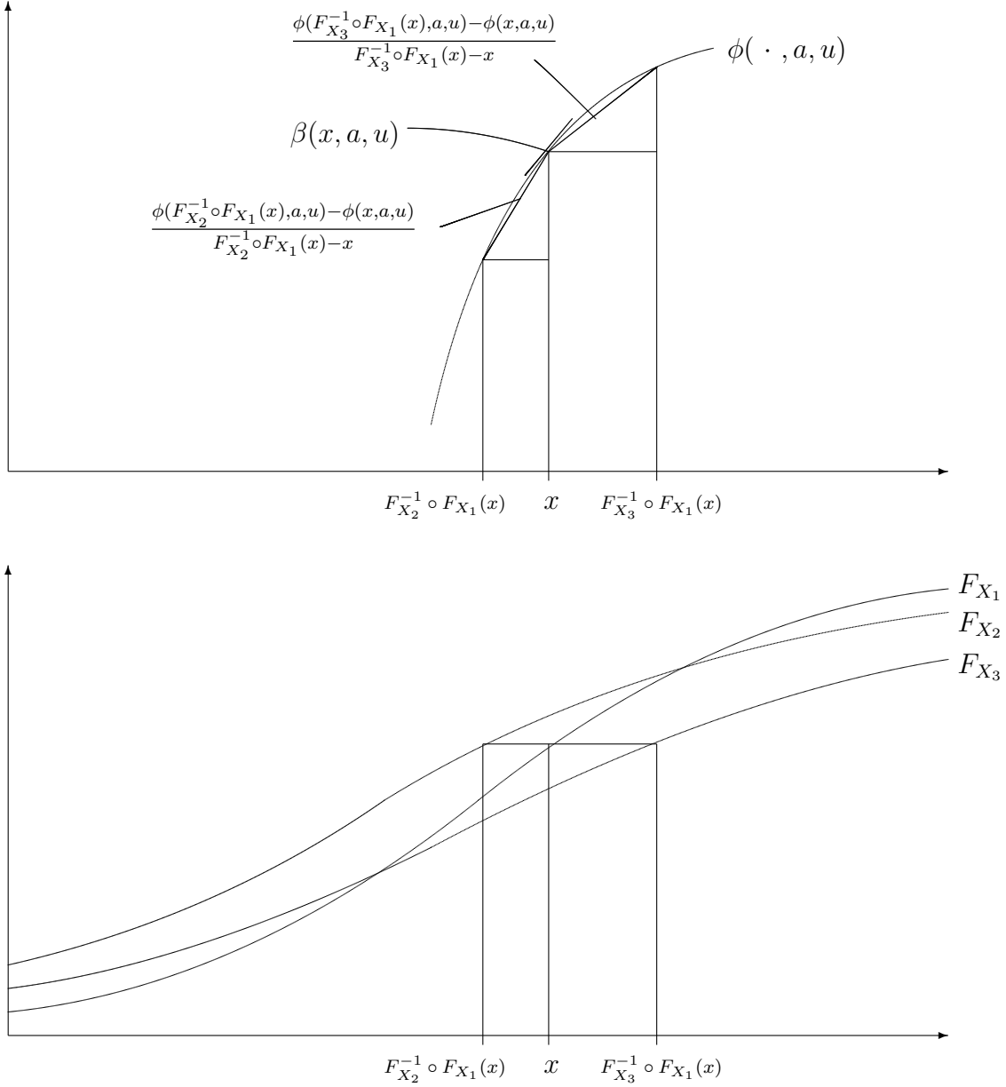
Figure 1: Partial identification under T < \infty : difference quotients form bounds of \beta(x, a, u) .
