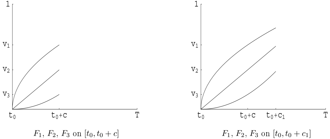
Figure 3. Solution to the main problem on [t_0, t_0 + c] (left) and extended solution to the main problem on [t_0, t_0 + c_1] (right).
