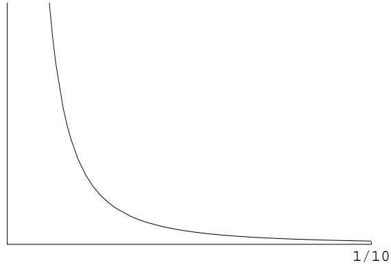
Figure 2. Function in (3.5).
