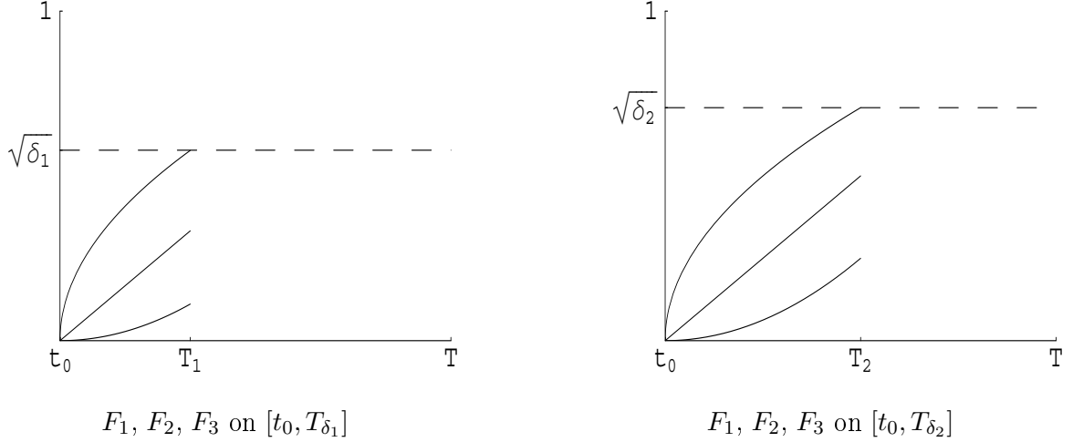
Figure 9. Maximal intervals of existence of a solution to the main problem: [t_0, T_{\delta_1}] corresponds to \delta_1 (left), [t_0, T_{\delta_2}] corresponds to \delta_2 , where \delta_2 > \delta_1 (right).
