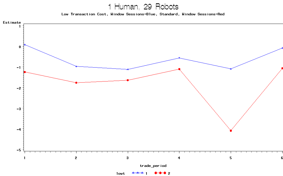
Figure 14: Random Effects by Experiment, Transaction Cost Treatments
