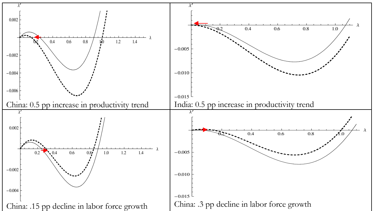
Figure 2: Long-run dynamics
