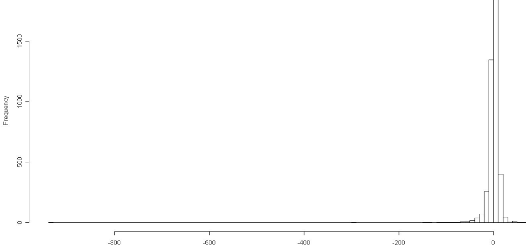
Figure 2: Residual Distribution (Non-Trimmed Data; OIA)
