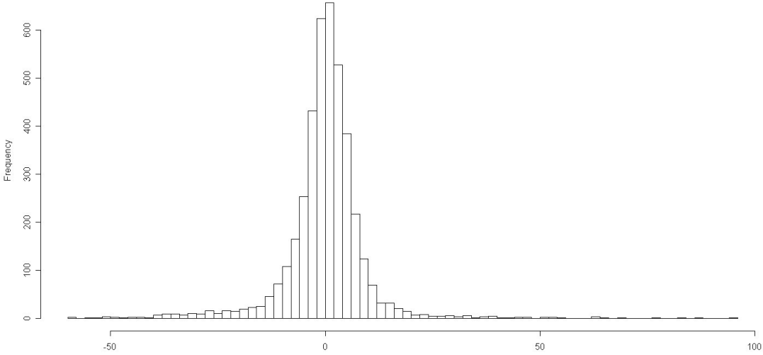
Figure 3: Residual Distribution (Trimmed Data; NIA)
