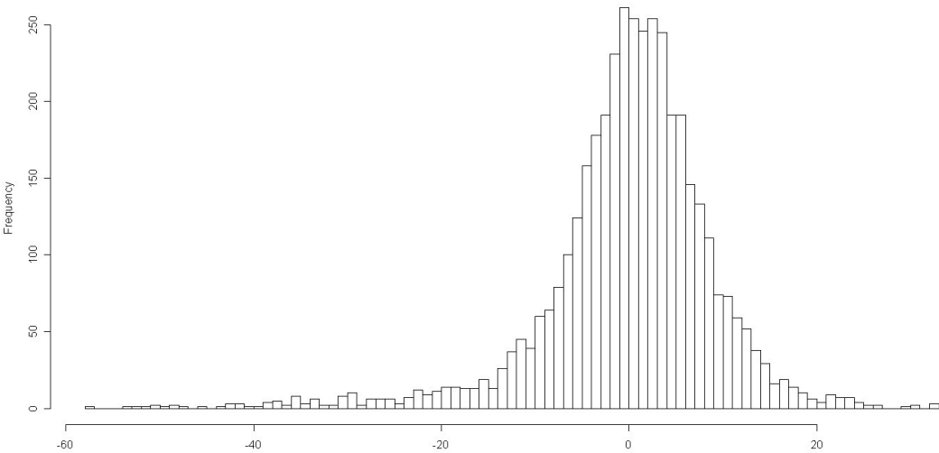
Figure 4: Residual Distribution (Trimmed Data; OIA)
