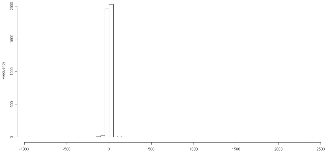
Figure 1: Residual Distribution (Non-Trimmed Data; NIA)
