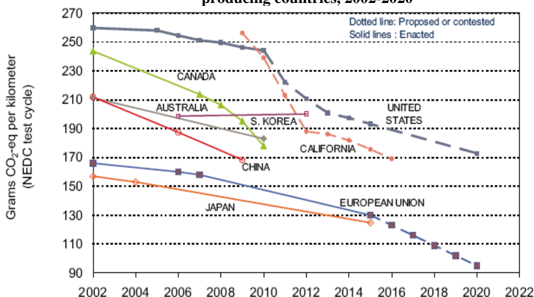
Figure 21. Actual and projected CO 2 emissions for new passenger vehicles, by major auto-producing countries, 2002-2020
