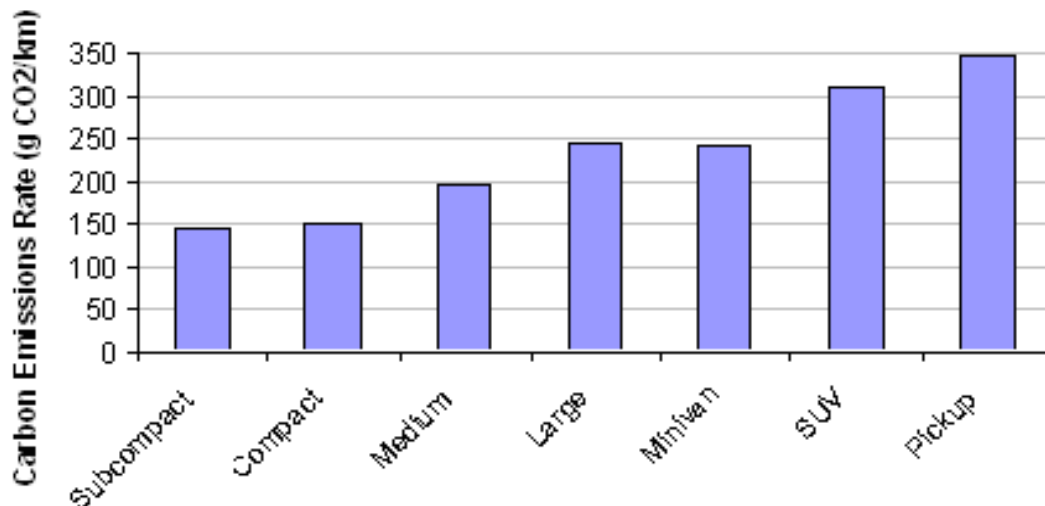
Figure 18. Average CO 2 emission rate by automobile segment, 2002
