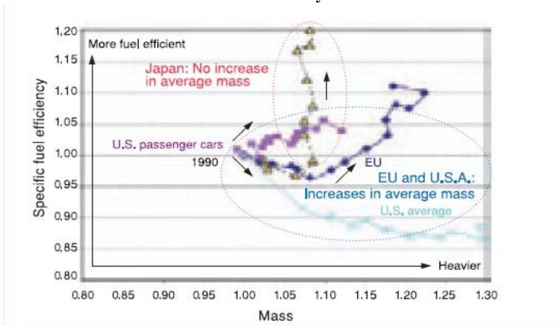
Figure 17. International comparison in passenger car weight: Vehicle fuel efficiency and mass
