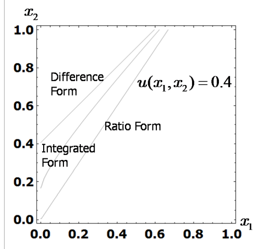
Figure 1: Comparison of contest success functions. Each line shows the combinations of x_1 and x_2 where side 1's probability of winning is 0.4. We use the values, \kappa = 1, \rho = 0.3
