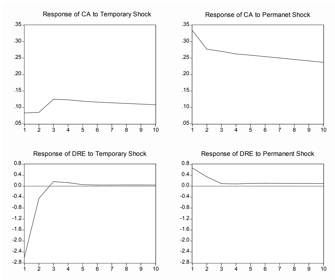
Figure 1A. USA: Impulse Response, estimated over the whole sample period
