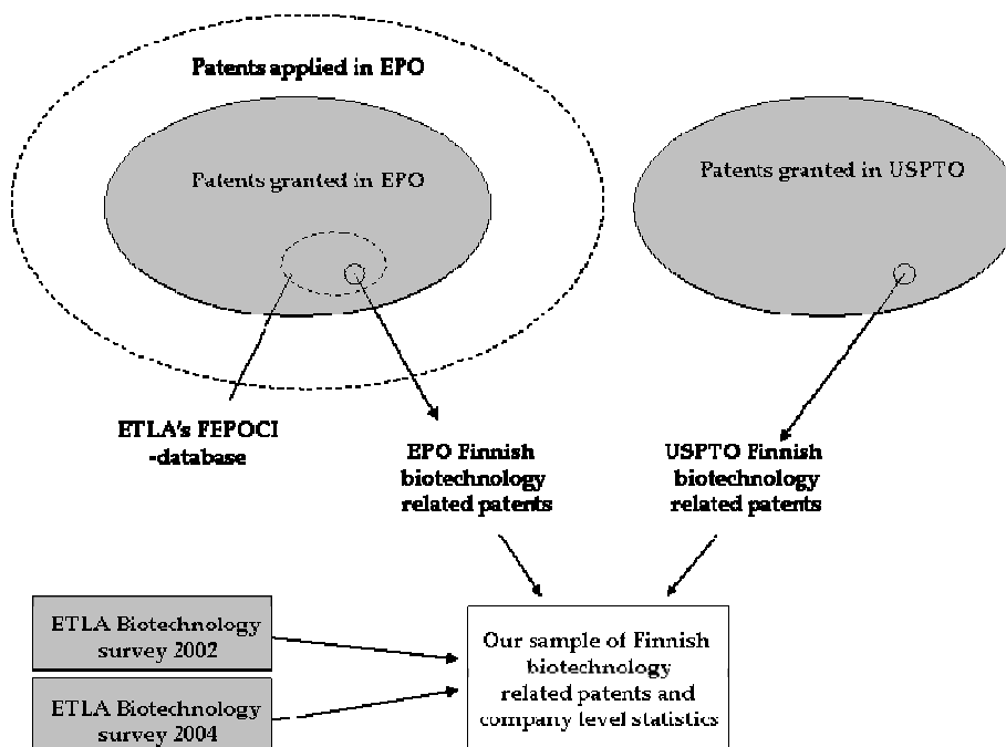
Figure 2. Data construction
