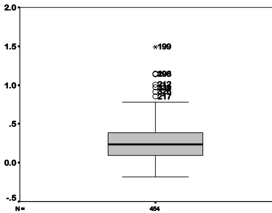
Figure 7 Comparison of boxplot graphs for selected variables
