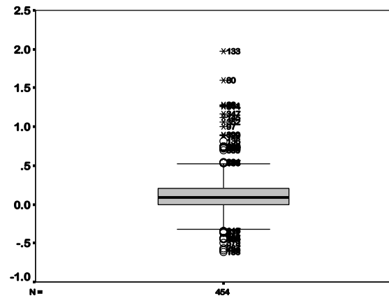
Figure 7 Comparison of boxplot graphs for selected variables
