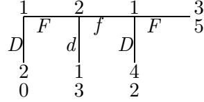
FIGURE 1. A centipede game
