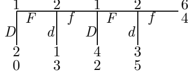
FIGURE 2. A four-legged centipede game
