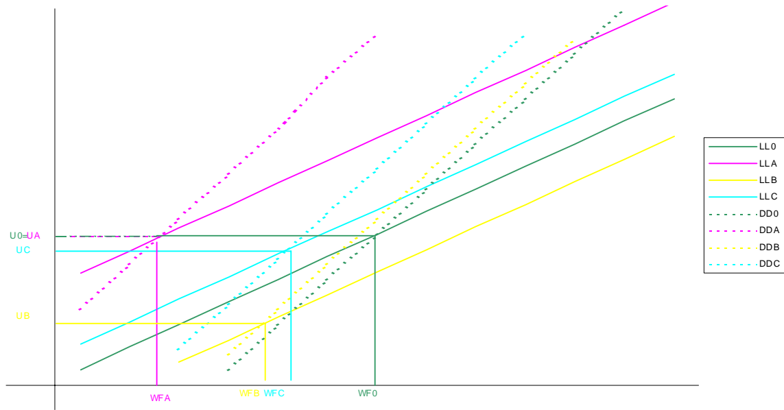
Figure 3: The Labour market loci (LL) and Trade balance loci (DD) in Case 0 (benchmark), Case A, Case B and Case C
