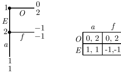
FIGURE 1. \Gamma_1 and its strategic form.
