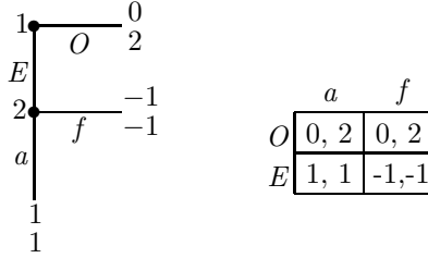
FIGURE 1. \Gamma_1 and its strategic form.
