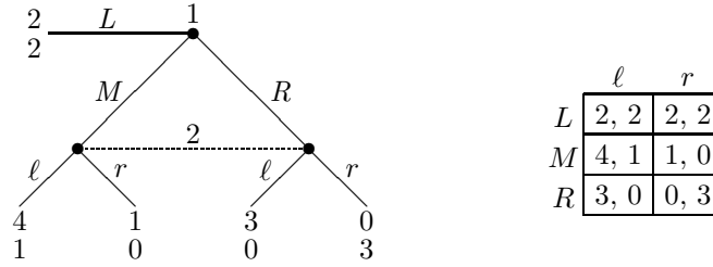
FIGURE 5. \Gamma_5 and its strategic form.
