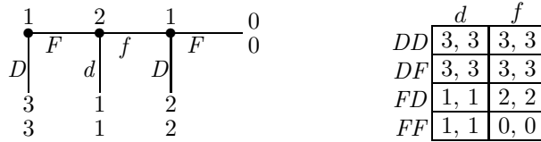
FIGURE 7. \Gamma_7 and its strategic form.
