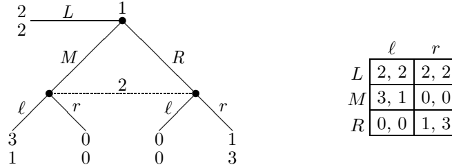
FIGURE 6. \Gamma_6 (= BoSwOO) and its strategic form.
