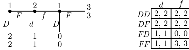
FIGURE 2. \Gamma_2 and its strategic form.
