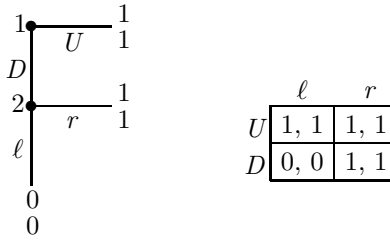
FIGURE 4. \Gamma_4 and its strategic form.
