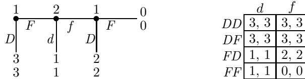
FIGURE 7. \Gamma_7 and its strategic form.
