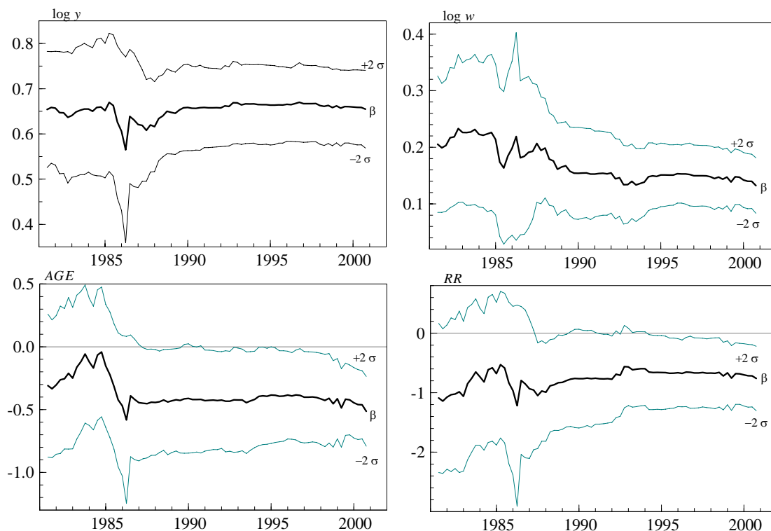
Figure 3: Recursive estimates of the coefficients of the extended cointegrated consumption function, with \pm 2 standard errors, denoted \sigma . Full sample estimates correspond to results in equation (3).
