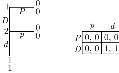
FIGURE 4. \Gamma_1 and its PRSF.
