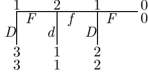
FIGURE 2. \Gamma_2
