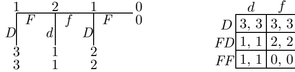
FIGURE 5. \Gamma_2 and its PRSF.
