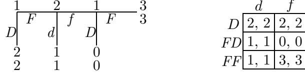
FIGURE 7. \Gamma_4 and its PRSF.
