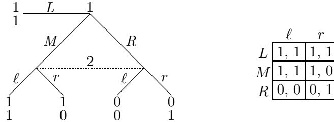
FIGURE 6. \Gamma_3 and its PRSF.
