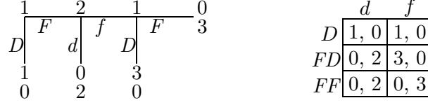
FIGURE 8. \Gamma_5 (= \text{TOL}(3)) and its PRSF.
