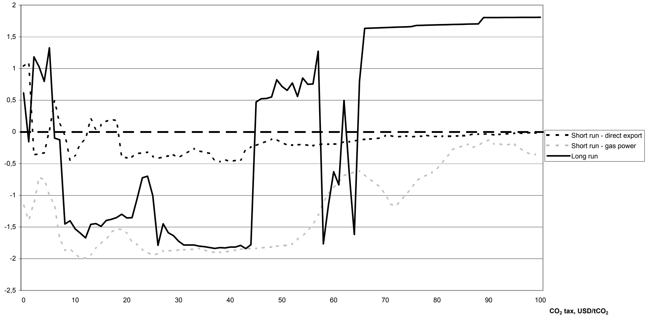
Figure 3 Net increase in total emissions of CO 2 in model countries following from increased extraction of natural gas in Norway (0.88 mtoe). Uniform CO 2 tax.
