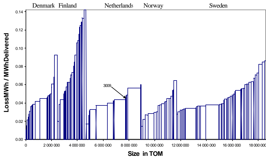
Panel c. Loss in MWh on MWh delivered
