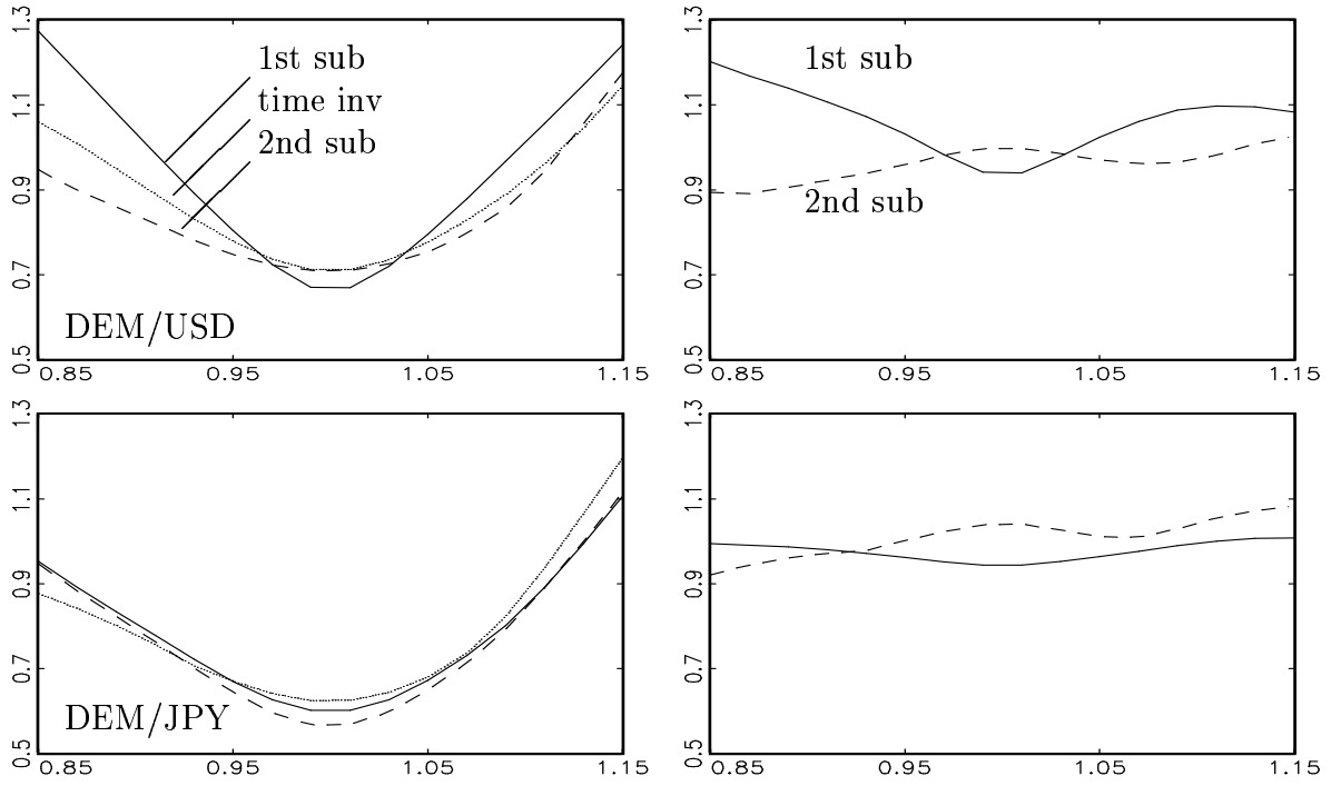
Figure 4: Implied volatilities (left hand side patterns) estimates for GARCH option prices with FX-rates as underlying assets. Time invariant and time varying GARCH-specifications are distinguished. Right hand side: Measures for two subsamples relative to the time invariant model. The x-axis is the moneyness S_0/K of the option, S_0 = 1 .
