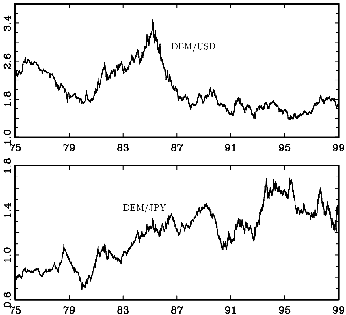
Figure 1: Log FX-rates
