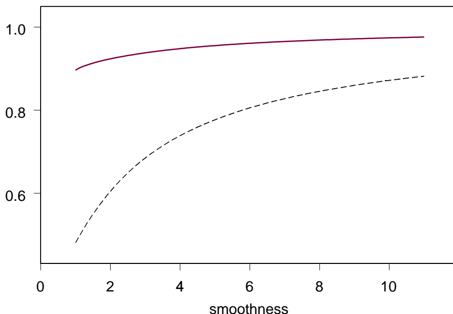
Figure 1: Minimax efficiency as function of the smoothness \beta (solid line: minimax efficiency of the spline method, dash line: minimax efficiency of the projection estimator).
