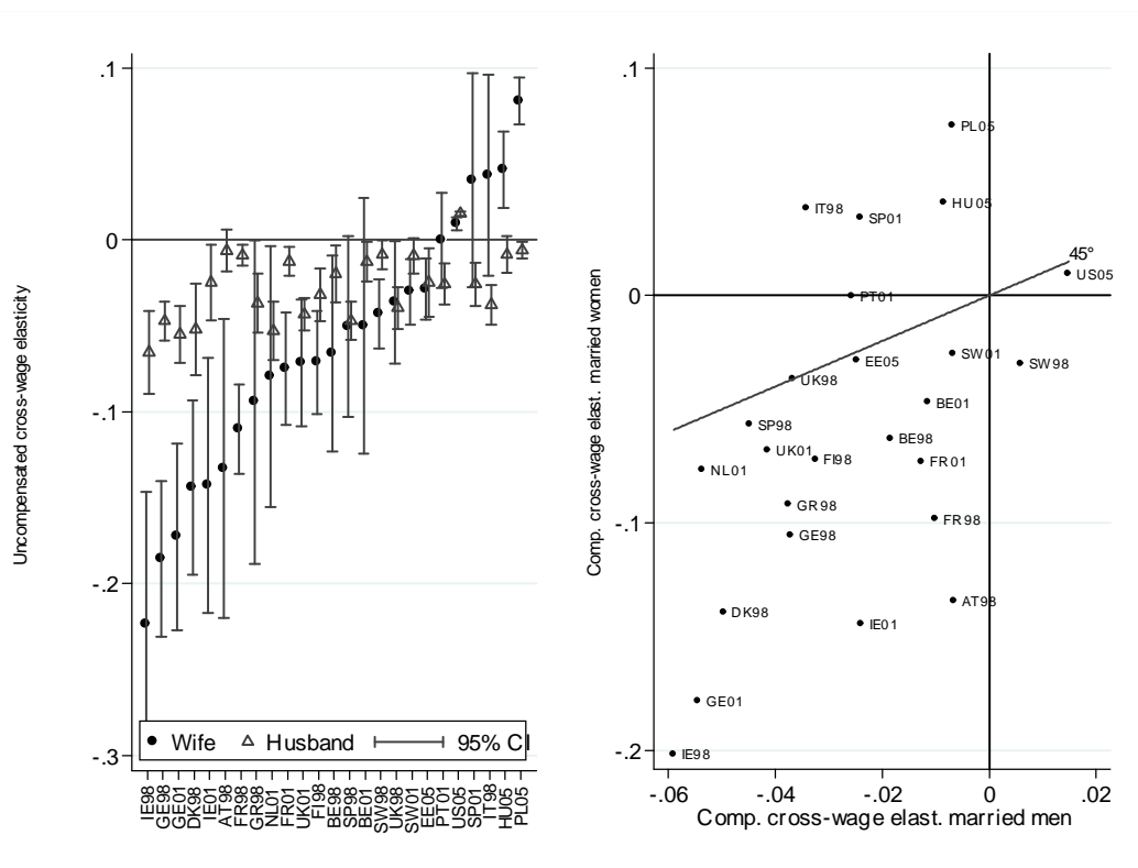
Figure 5: Cross-wage Elasticities
