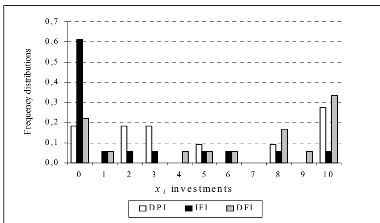
Figure 4: Frequency distributions of x_i -investments for DPI , DFI and IFI treatment.
