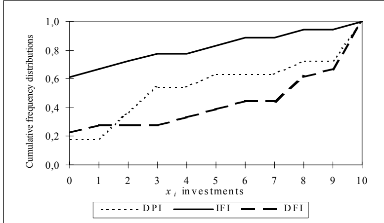
Figure 5: Cumulative frequency distributions of x_i -investments for DPI , DFI and IFI treatment.
