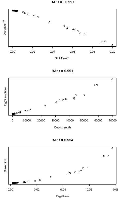
Figure 4: Relationship between disruption and centrality measures in BA networks
