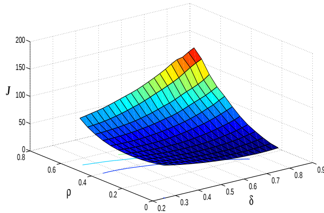
Figure 5: 3-D contour plot of the parameter space with \delta and \rho
