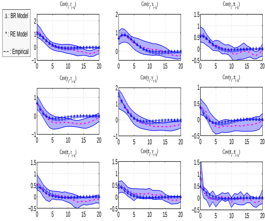
Figure 2: Model covariance (Cov) profiles in the Euro Area.
