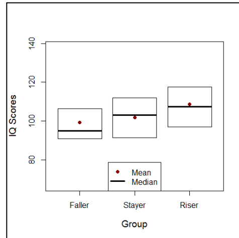
Figure 9: IQ scores and Occupational Mobility
