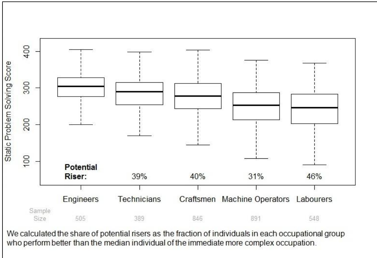
Figure 2: Static Problemsolving Skills for four different technical occupational groups in Canada
