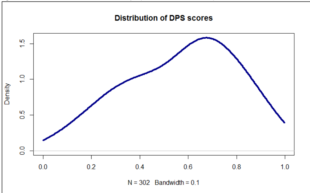
Figure 11: Distribution of DPS scores in our sample (Gaussian kernel estimator)
