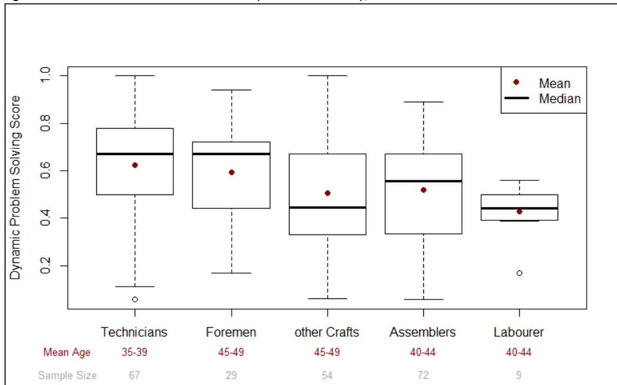
Figure 3: DPS skills for different technical occupations in Germany, 2011
