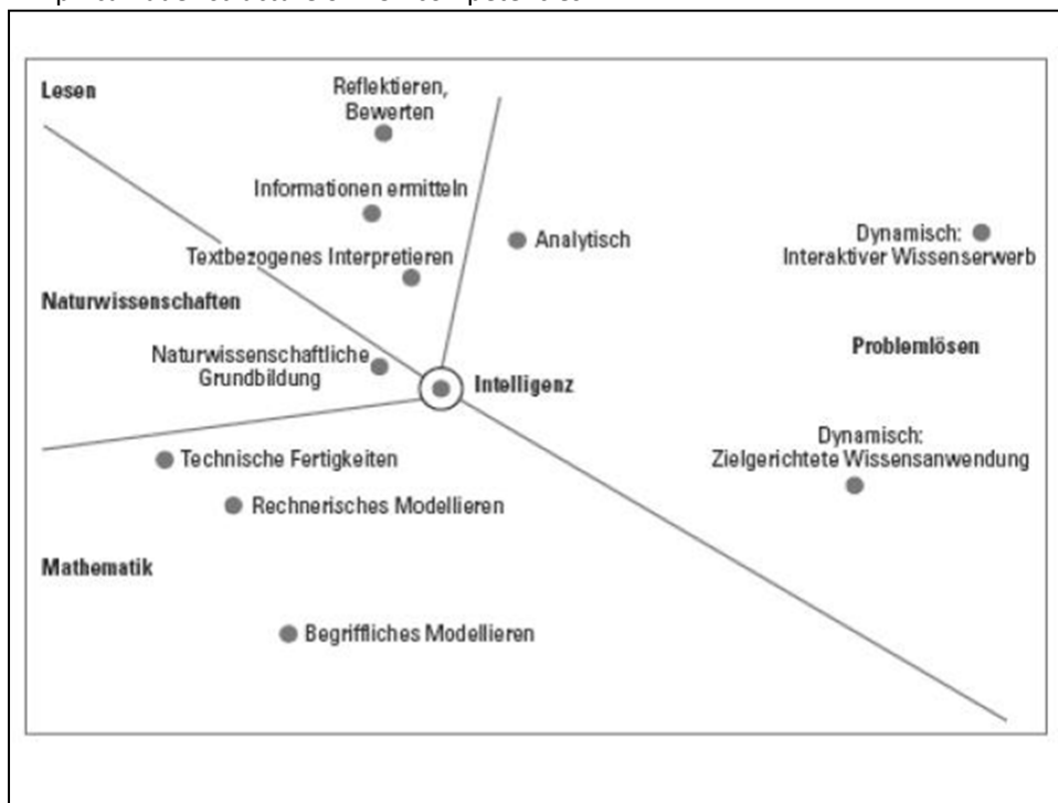
Figure 10: Empirical radex structure of PISA competencies
