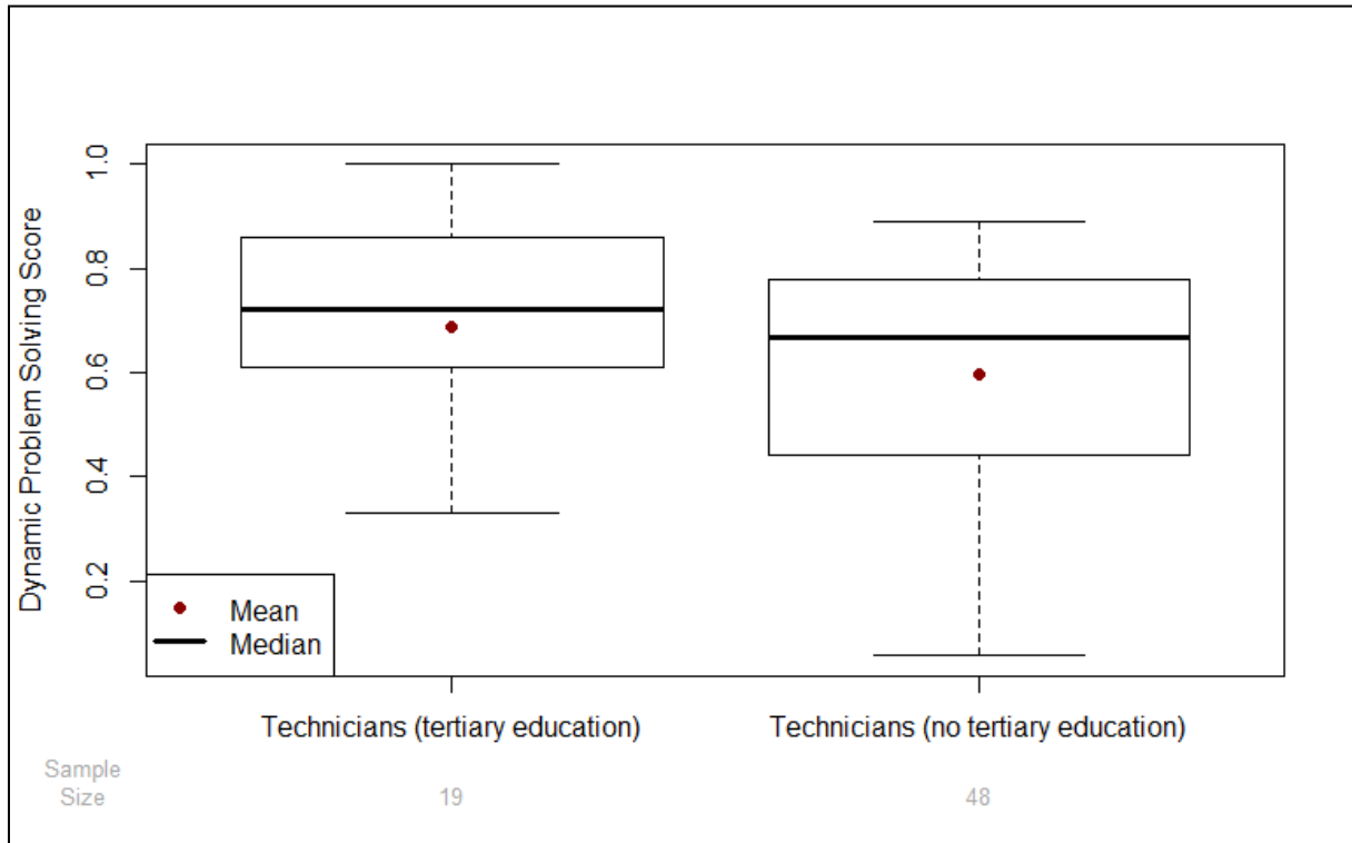
Figure 5: DPS scores for technicians with or without tertiary education
