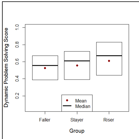
Figure 8: DPS scores and Occupational Mobility
