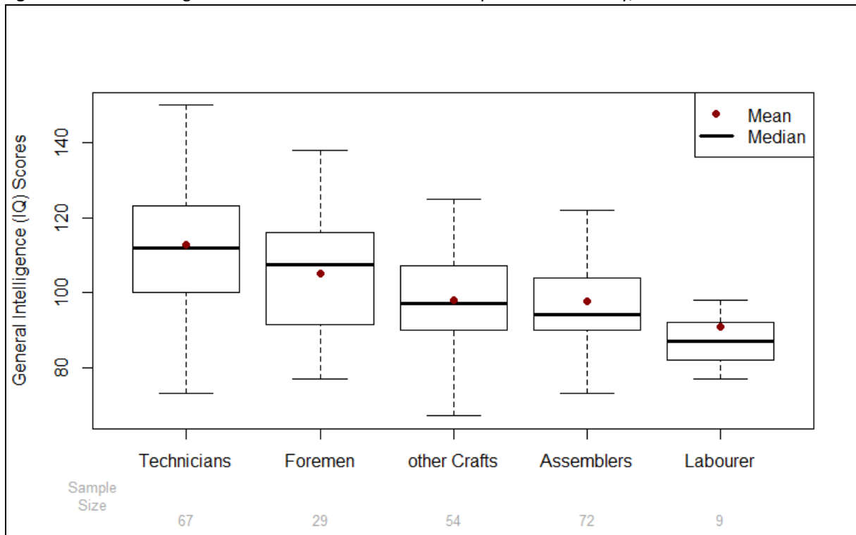
Figure 4: General Intelligence Skills for different technical occupations in Germany, 2011
