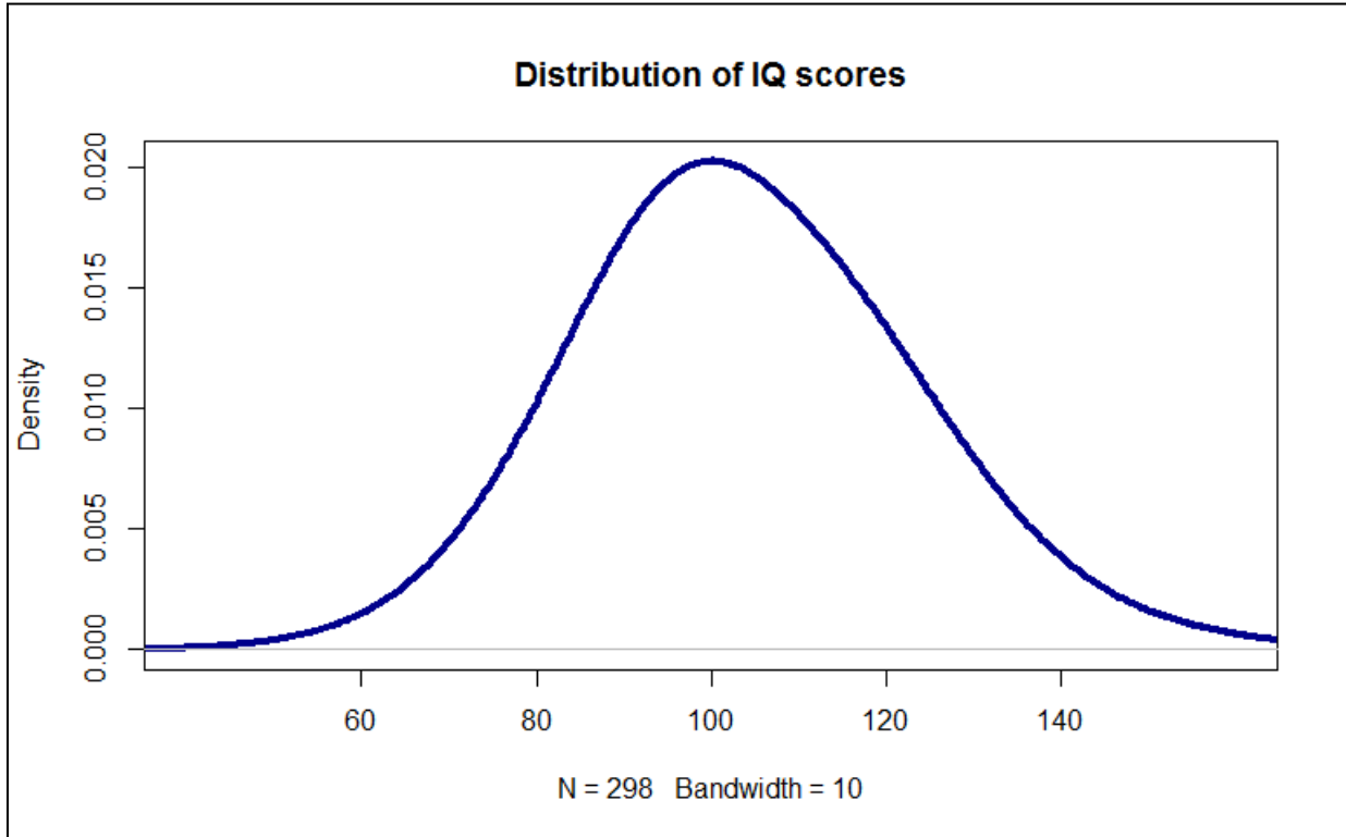
Figure 12: Distribution of general intelligence scores in our sample (Gaussian kernel estimator)
