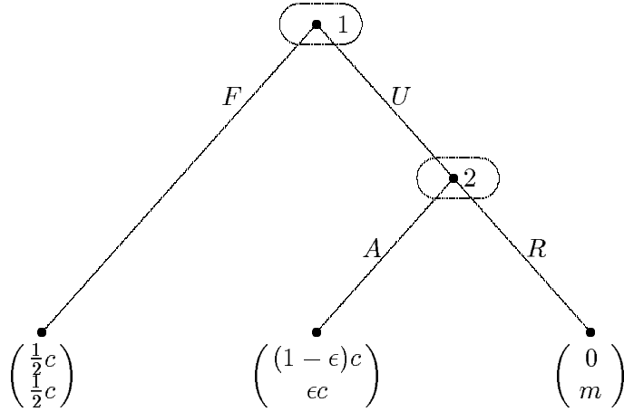
Figure 2.1: "Ultimatum Minigame"
