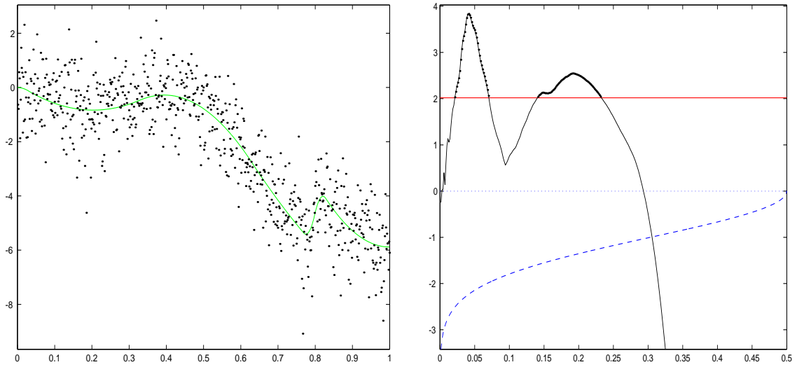
Figure 5: Simulated data with f \notin \mathcal{H}_\downarrow and \tilde{T}_n(\vec{Y}, \cdot)
