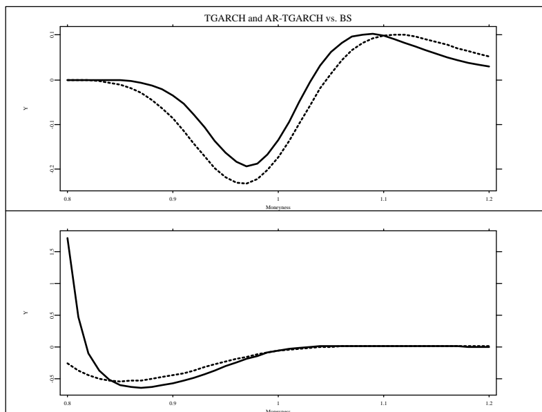
Figure 4: Upper panel: Difference between simulated TGARCH option prices to Black and Scholes prices. TGARCH parameters were set to \alpha = 0.03 , \alpha^- = 0.12 , \beta = 0.9 . The x-axis represents the moneyness of the option. The dashed line incorporates AR(1) dynamics ( \phi = 0.2 ), the solid one does not. Lower panel: the corresponding differences divided by the Black and Scholes price.
