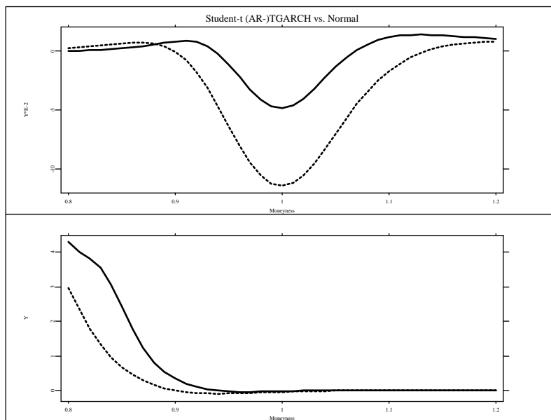
Figure 6: Upper panel: Difference between simulated TGARCH option prices with Student-t innovations to GARCH prices with normal innovations. TGARCH parameters were set to \alpha = 0.03 , \alpha^- = 0.12 , \beta = 0.9 and the Student-t degrees of freedom to \nu = 6.4 . The x-axis represents the moneyness of the option. The dashed line incorporates AR(1) dynamics with \phi = 0.2 , the solid one does not. Lower panel: the corresponding differences divided by the (AR-) GARCH price with normal innovations.
