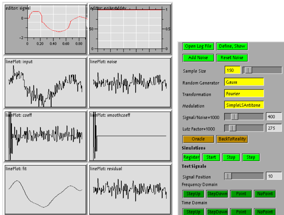
Figure 4: Simulation for REACT. Only minimal custom components need to be added. Re-usable components for display ...for control: just re-used software components! Plugged-in generic ON transformation Plugged-in custom Stein shrinkage (Dümbgen, 1998)
