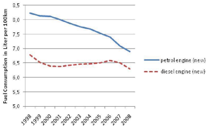
Figure 3: Average Fuel Efficiencies of Newly Registered Diesel and Petrol Cars in Germany (BMW1, 2011).
