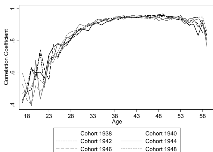
Figure 3: Rank correlations of consecutive years for cohorts 1938-1948.
