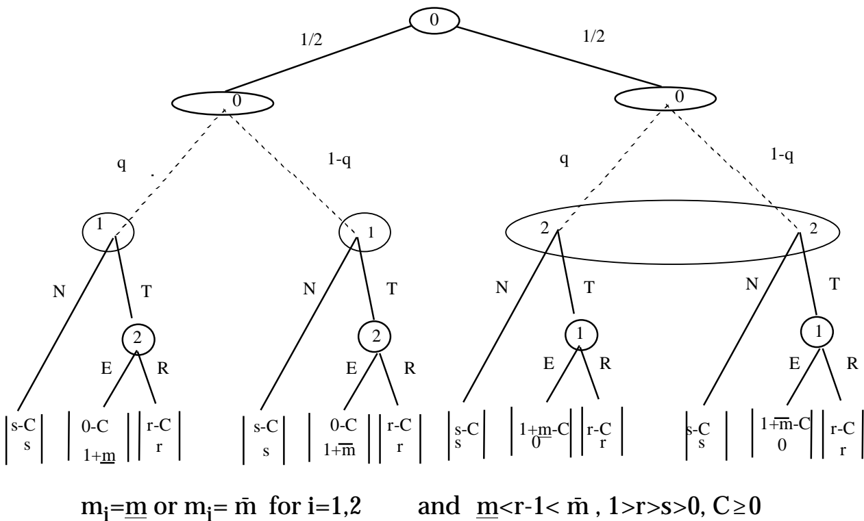
I-type player 1 and U-type player 2
