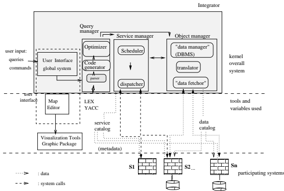
Fig. 1. The generic open GIS architecture
