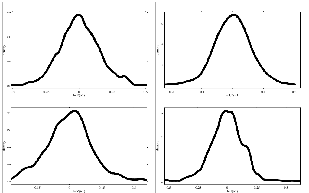
Figure 1e: Density estimates for 1996, upper left: \ln F_{i,t-1} , upper right: \ln U_{i,t-1}^* , lower left: \ln V_{i,t-1} , lower right: \ln I_{i,t-1}
