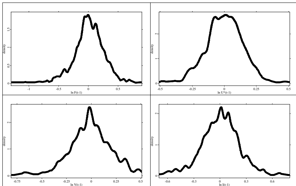
Figure 1a: Density estimates for 1992, upper left: \ln F_{i,t-1} , upper right: \ln U_{i,t-1}^* , lower left: \ln V_{i,t-1} , lower right: \ln I_{i,t-1}
