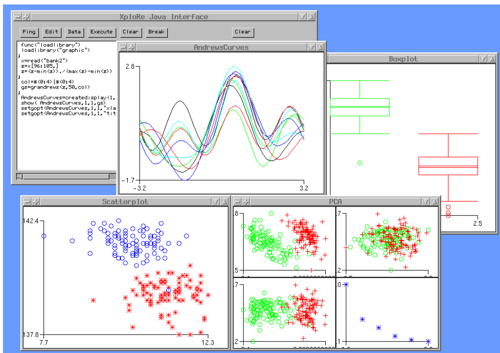
Figure 8: Graphical exploration of Swiss bank notes data
