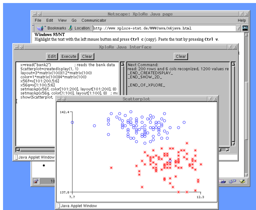
Figure 2: Screenshot of the XploRe Java version
