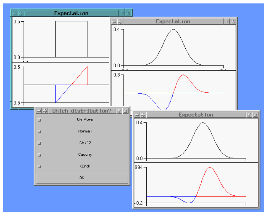
Figure 6: Graphical demonstration of expectation
