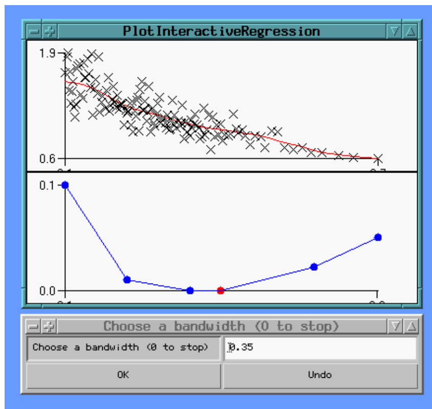
Figure 10: Fitting a kernel regression interactively
