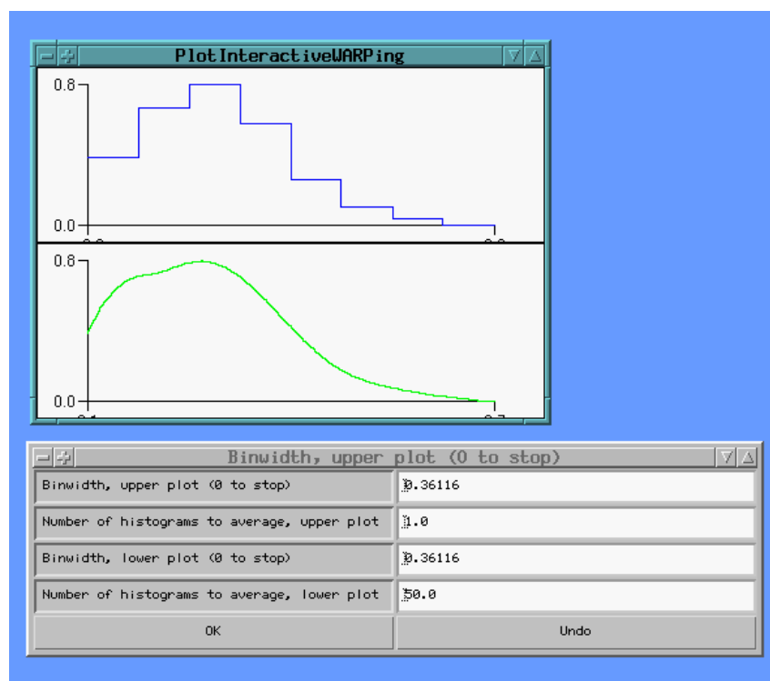
Figure 9: Comparing averaged shifted histograms w.r.t. their parameters
