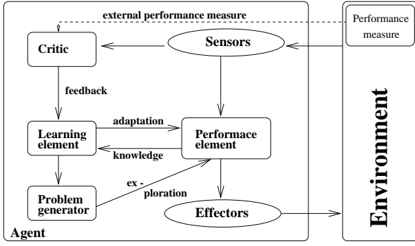
Fig. 2. Conceptual learning agent architecture according to Russell & Norvig (adapted from [RN95]).
