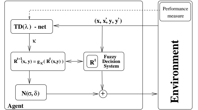
Fig. 3. Reinforcement-driven fuzzy-relation-adaptation architecture.
