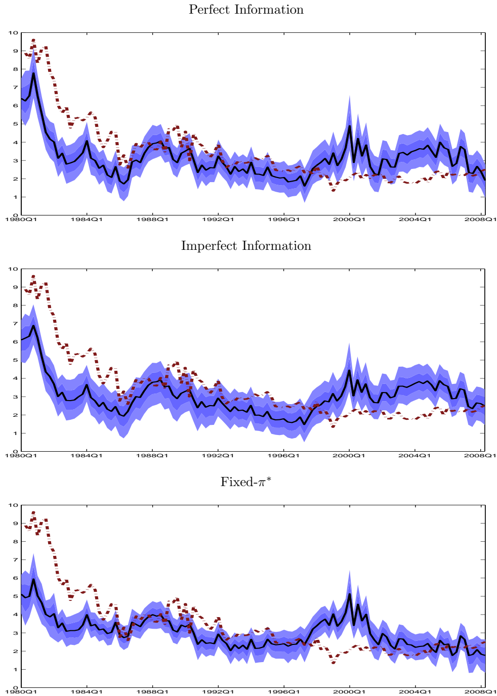
Figure 5: Inflation Expectations: Data vs Model Prediction, 1980-2008 Sample
