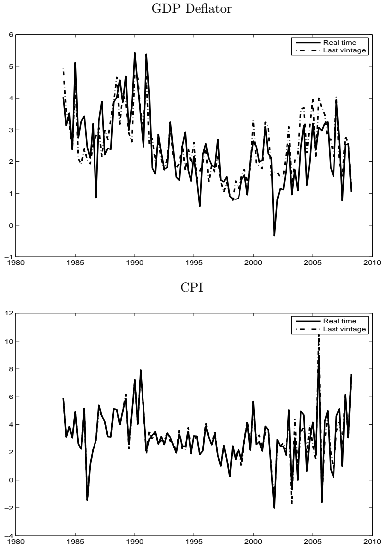
Figure A.1: Revisions in Inflation Data: Real Time vs Last Vintage
