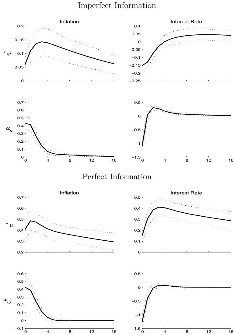
Figure A.2: Impulse Responses (Dataset with Inflation Expectations)
