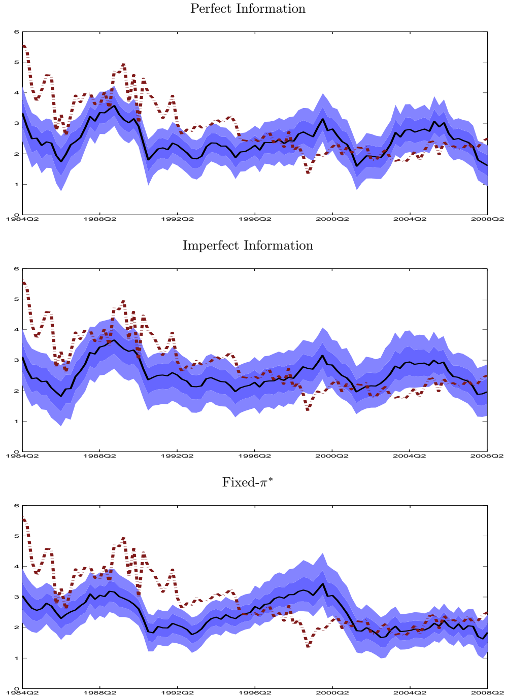
Figure 1: Inflation Expectations: Data vs Model Prediction
