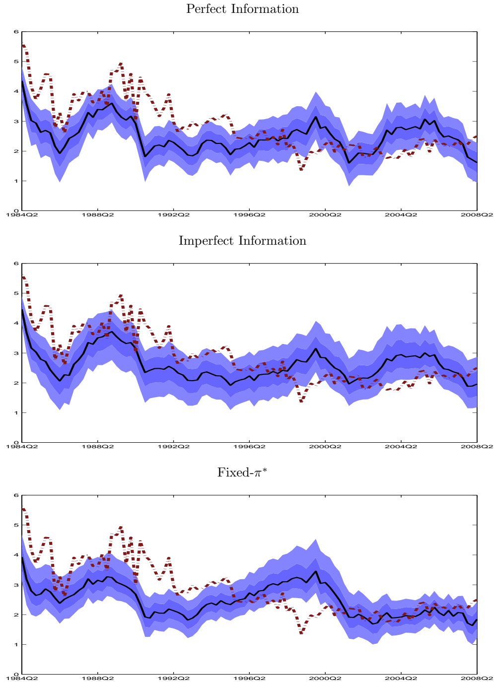
Figure A.3: Inflation Expectations: Data vs Model Prediction, Conditioning on Initial Observation for Inflation Expectations
