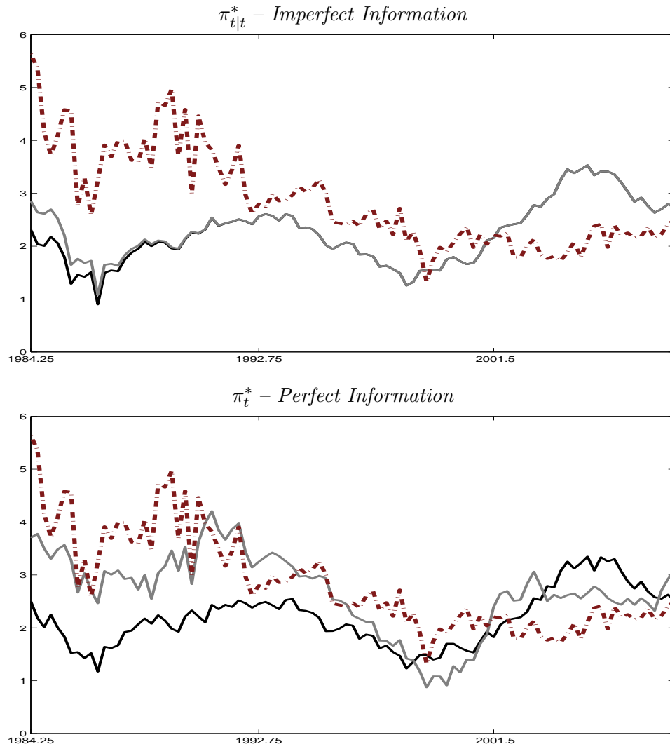
Figure 2: \pi_t^*
