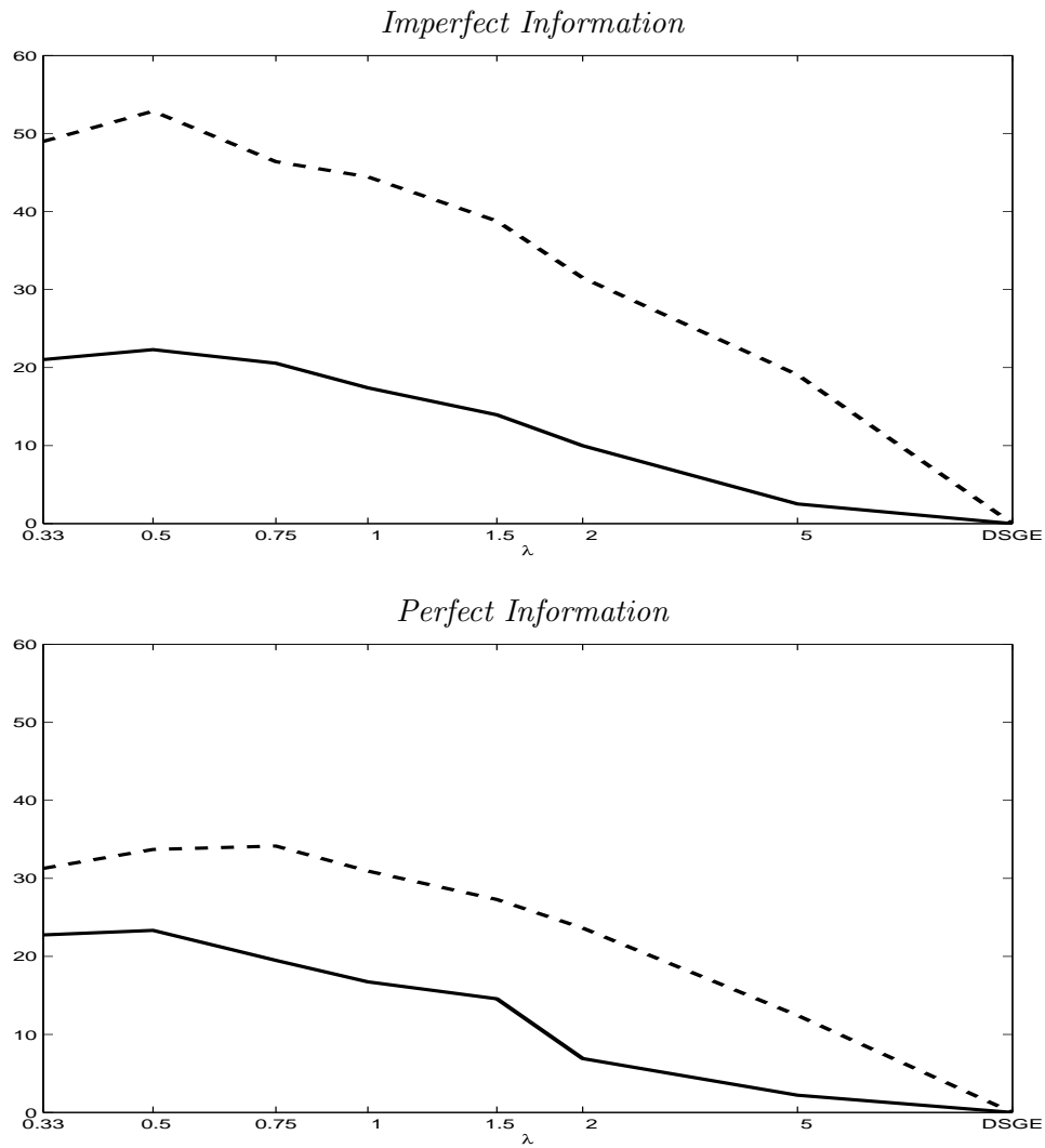
Figure 3: DSGE vs VARs
