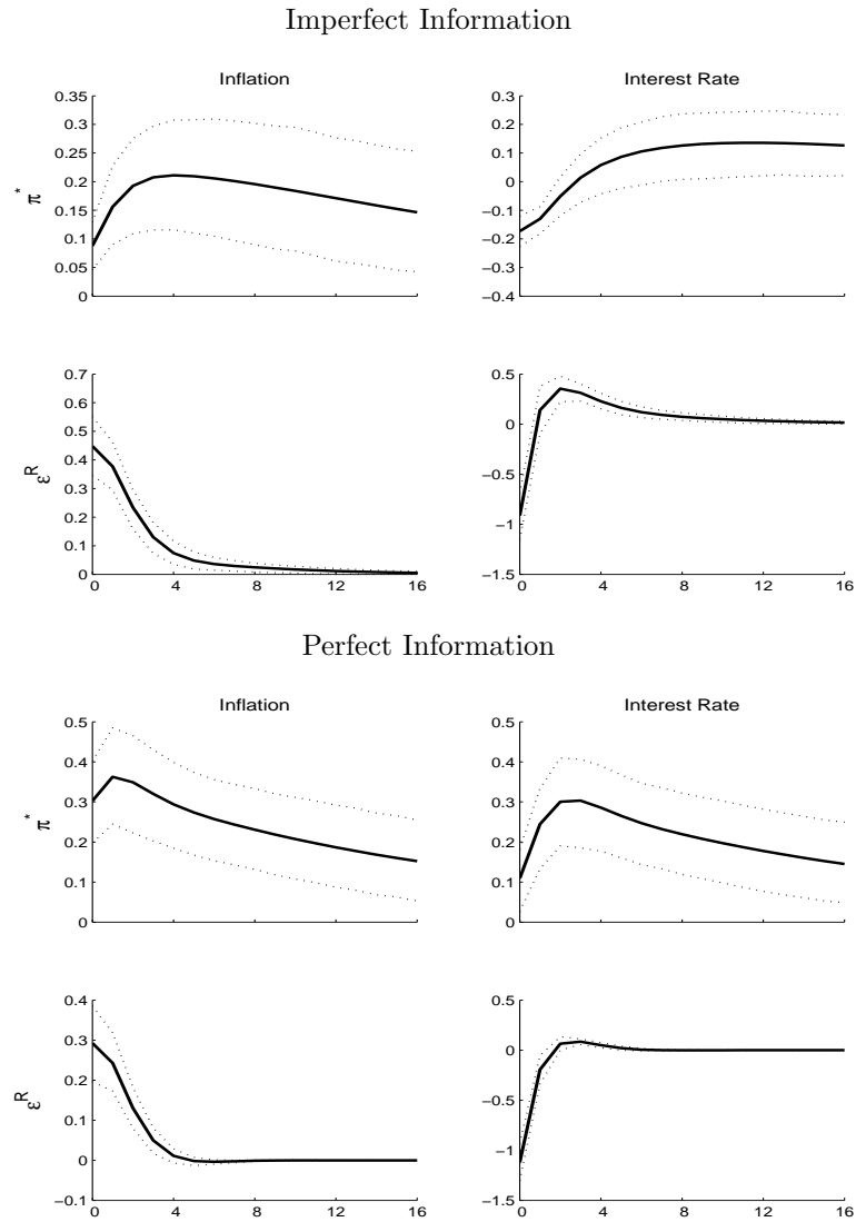
Figure 4: Impulse Responses
