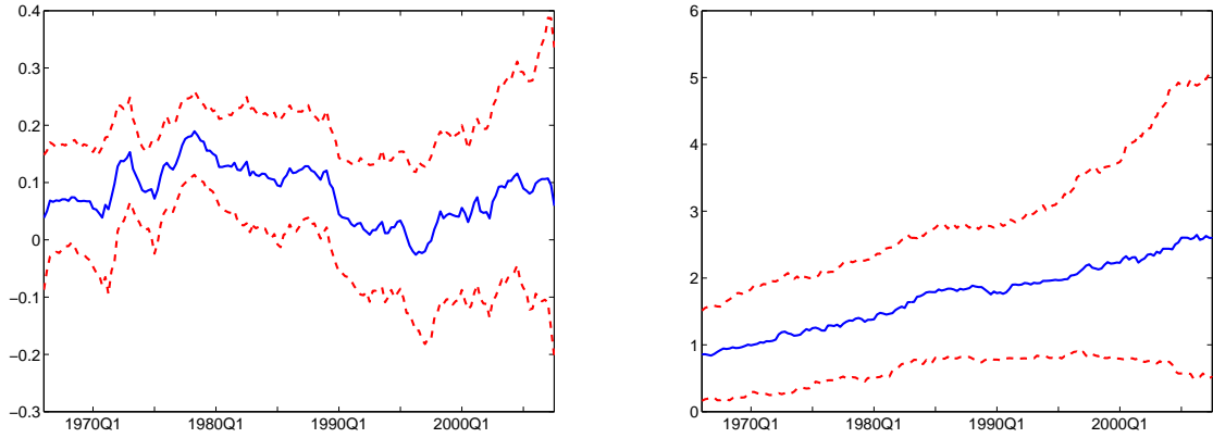
Figure 1: Posterior densities of selected \beta parameters in BMASB Phillips curve model (6) for h = 1 conditional on inclusion: PCE Deflator Inflation
