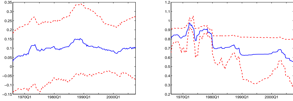
(b) BMASB Persistence – TVP-AR Persistence
