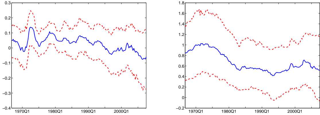
Figure 4: Posterior densities of selected \beta parameters in BMASB Phillips curve model (6) for h = 4 conditional on inclusion: GDP Deflator Inflation
