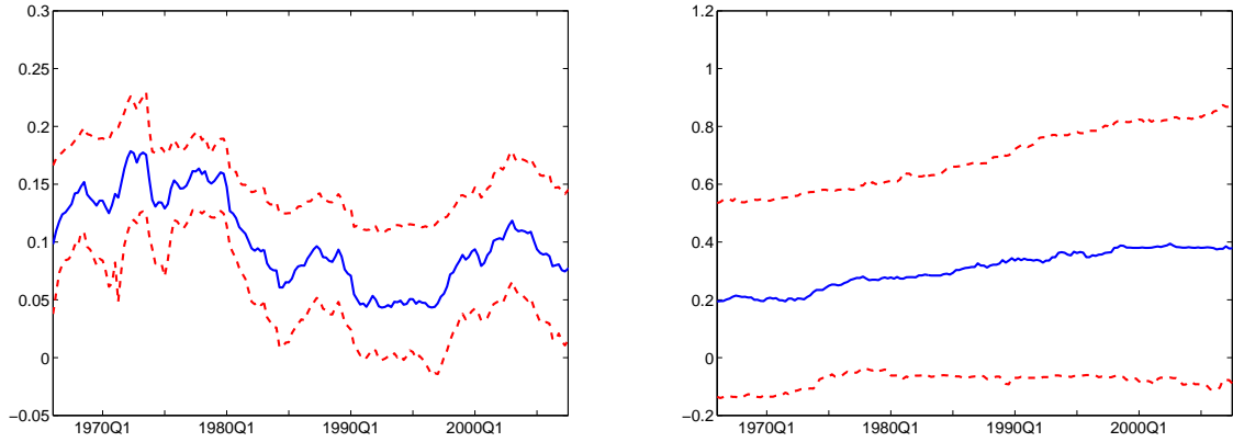
Figure 3: Posterior densities of selected \beta parameters in BMASB Phillips curve model (6) for h = 1 conditional on inclusion: GDP Deflator Inflation
