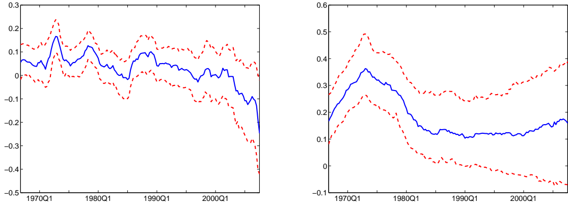
Figure 2: Posterior densities of selected \beta parameters in BMASB Phillips curve model (6) for h = 4 conditional on inclusion: PCE Deflator Inflation
