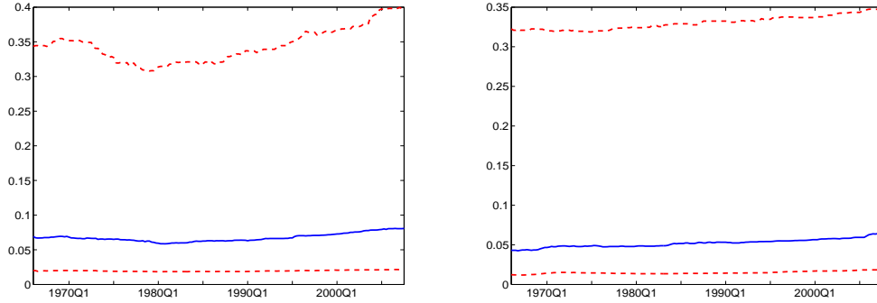
(c) BMASB \sigma_t^2 – TVP-AR \sigma_t^2
