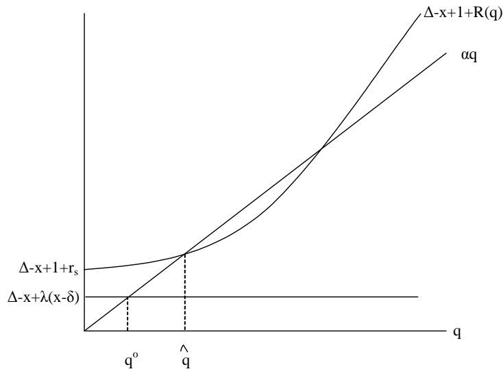
Figure 1: Excess risk taking: \hat{q} > q^o
