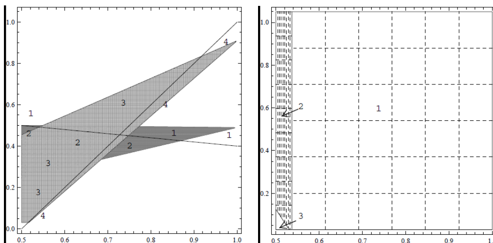
Figure 2: Comparing the equilibrium (left) and planner’s (right) allocations, when an LSM is not available. \mu is given on the X-axis and \gamma/R is given on the Y-axis. For these graphs we used \sigma = 0.15 and \theta = 0.6 . Left panel: equilibrium allocations. Right panel: planner’s allocations. The numbers correspond to the rows of Table 1.
