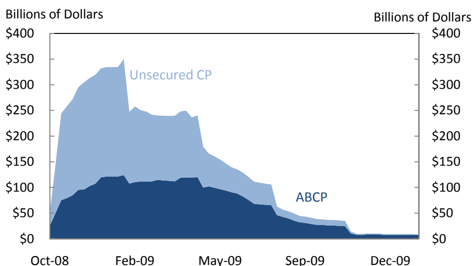
Figure 7: CPFF Outstanding
