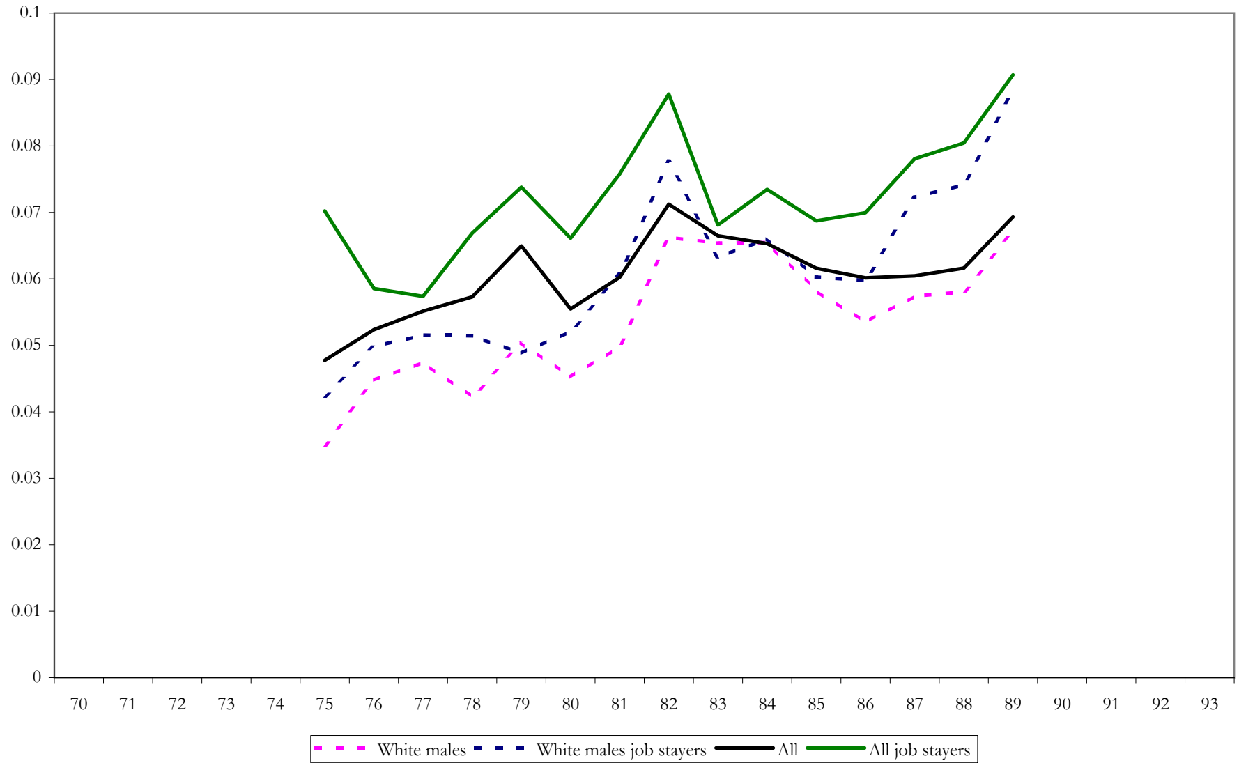
Figure 2: Persistent volatility of log real earnings in the PSID
