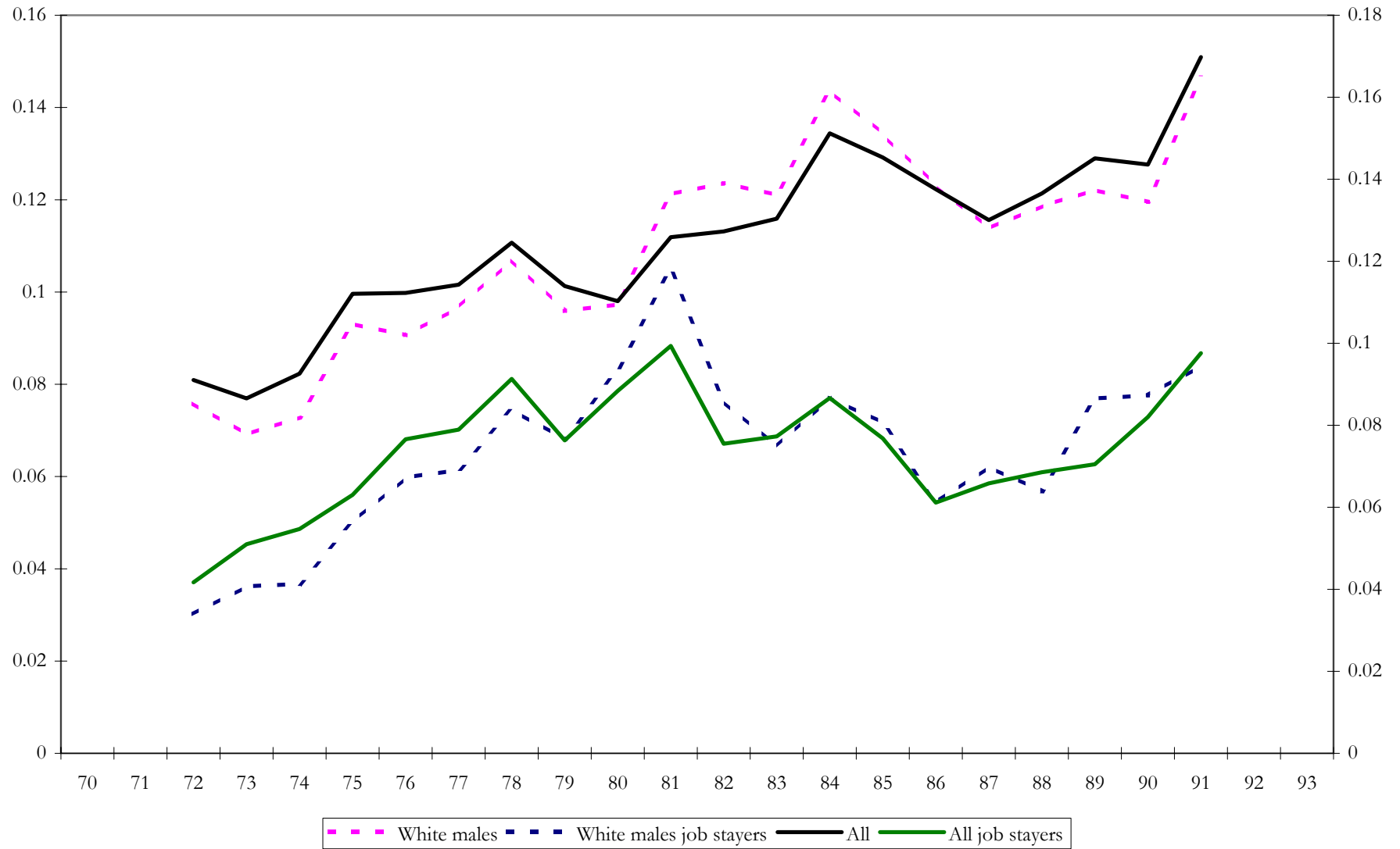
Figure 1: Very transitory volatility of log real earnings in the PSID
