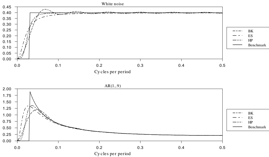
Figure 3. Frequency extraction problem with I(0) process
