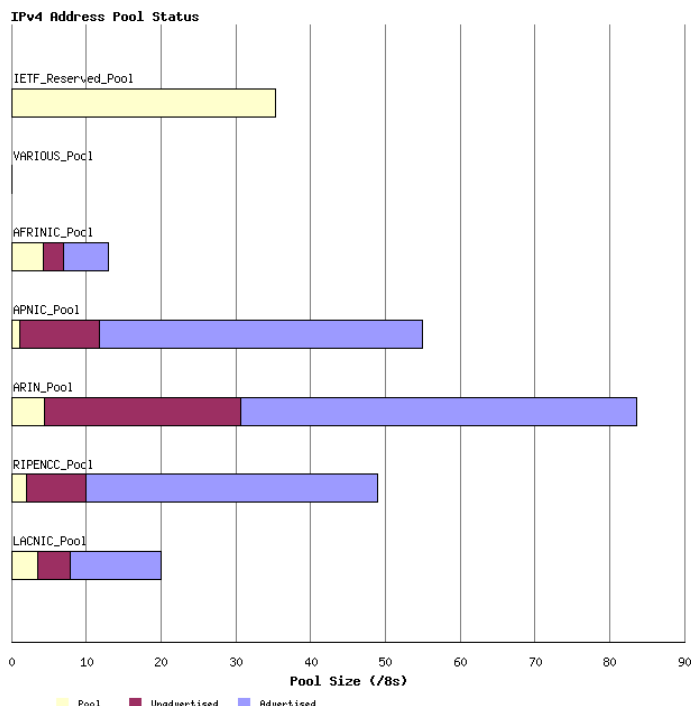
Figure 4: IPv4 address advertisement status 5
