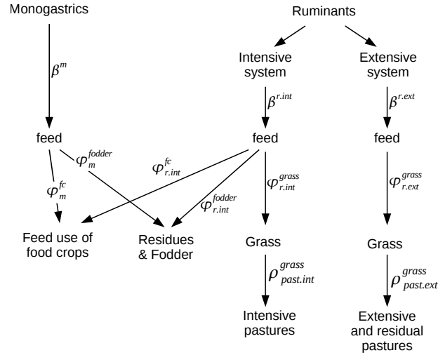
Figure 10: Links between animal calorie production, feed categories and pasture areas. Reading: the amount of feed required to produce one calorie of monogastric is \beta_m , split into a share \phi_m^{fc} of food crops and \phi_m^{fodder} of crop residues and fodder. Values are reported in tables 4, 5 and 6
