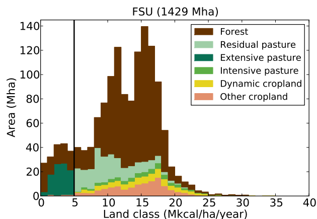
Figure 11: Illustration of the production frontier (limit land class j_{limit} ) on the histogram of the land area classes of potential yield in the Former Soviet Union (black vertical bar).
