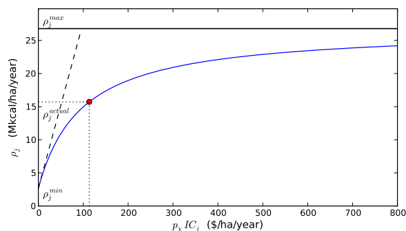
Figure 8: Yield in a land class as a function of chemical input consumption IC_j . \rho_j^{max} , \rho_j^{actual} and \rho_j^{min} are the potential, actual and minimum yields of the land class j . p_\chi is the price index of chemical inputs.
