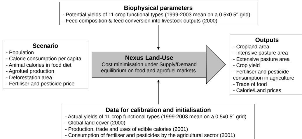
Figure 1: Description of the modelling system. “Fertiliser and pesticide consumption” includes also other consumption of chemical and mineral goods.
