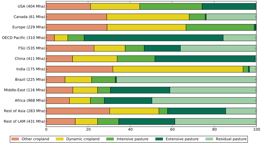
Figure 13: Share of different agricultural land-use types in the 12 regions of the model at the base year.
