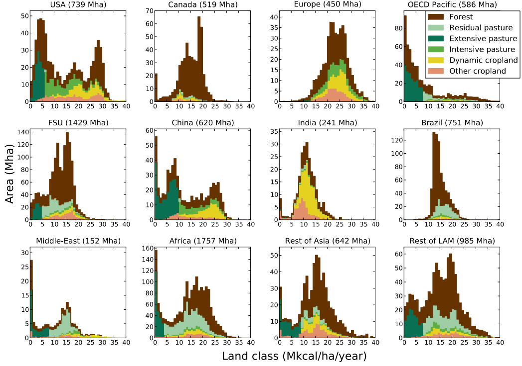
Figure 12: Histogram of the land area classes of potential yield in the 12 Nexus Land-Use regions at the base year.
