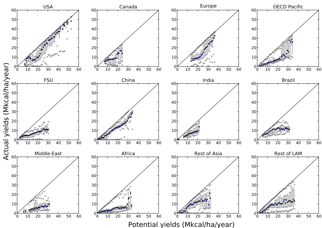
Figure 9: Actual yield versus potential yield of dynamic crops within each potential yield class. Crosses are minimums and maximums, whiskers go from the 20th to the 80th percentile. See figure 6 for a map of the difference between potential and actual yields of dynamic crops.
