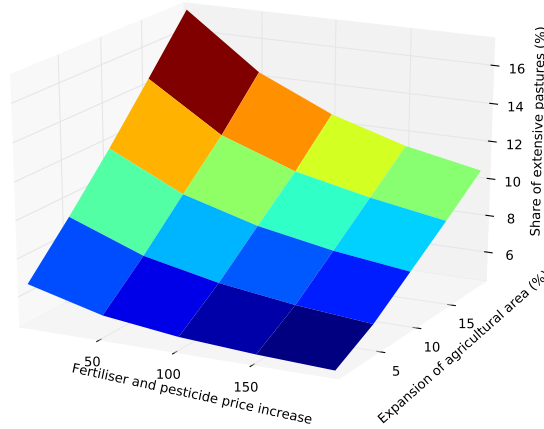
Figure 15: Variations of the proportion of extensive pastures in function of chemical inputs price and expansion rate of agricultural lands between 2001 and 2050.
