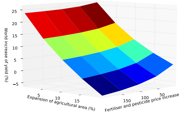
Figure 14: Variations of crop yields in function of chemical inputs price and expansion rate of agricultural lands 2001 and 2050.
