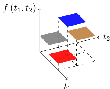
Figure 3 — The density function of a grid distribution.
