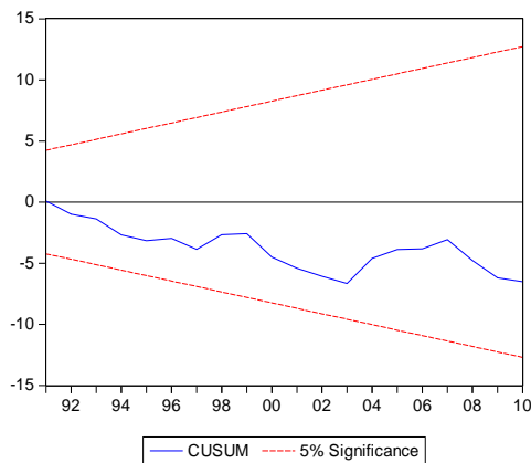
Figure 1. Cumulative sum of recursive residual
