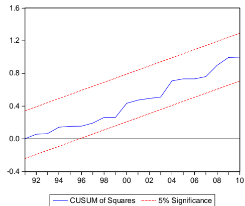
Figure 2. Cumulative sum of Square recursive residual
