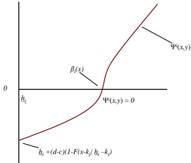
Figure 1: \Psi^i(x,y)
