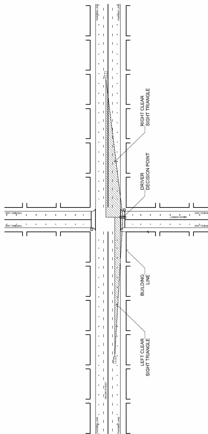
Figure 2.2: Left and Right Clear Sight Triangles
