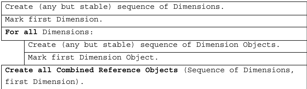
Figure 6: Recursive Algorithm for Calculation of set of Combined Reference Objects A runtime example of the above algorithm is shown in Figure 7.
