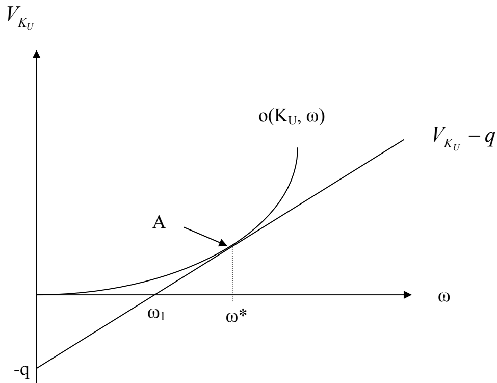
Figure 1: Smooth-Pasting Condition (Marginal investment condition)
